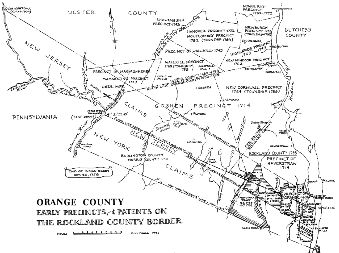
Figure 5 Minisink Patent 1734
